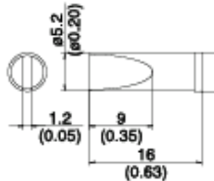
T12-DL52 SHAPE-5.2DL
