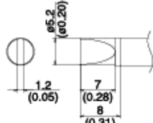
T12-DL32 SHAPE-3.2DL
