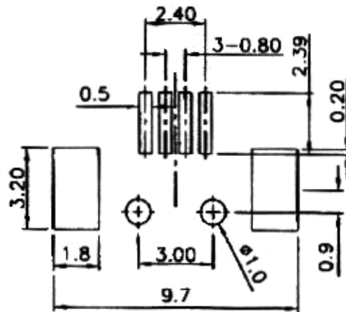
Recommard PCB Layout
