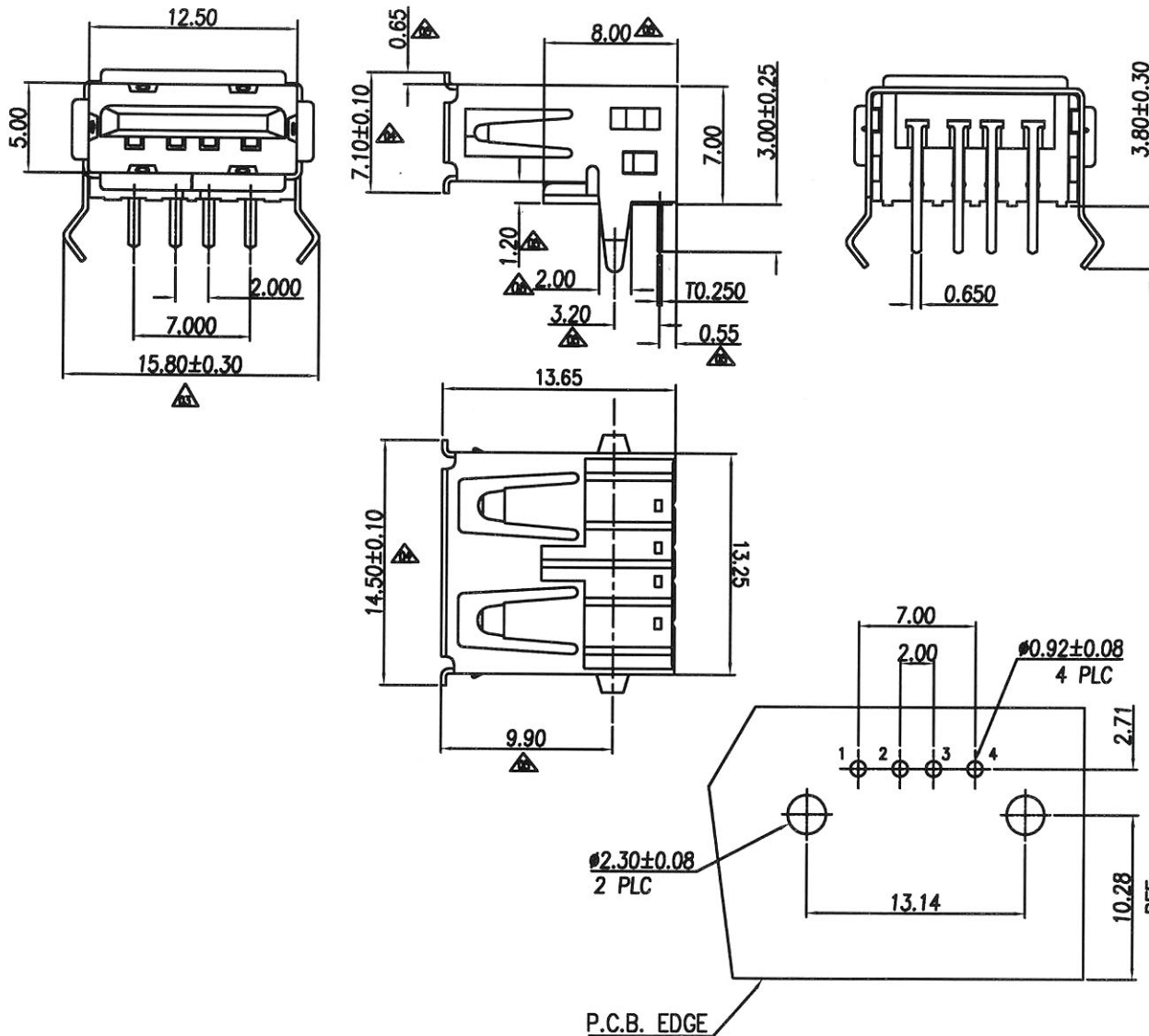
RECOMMEND P.C.B LAYOUT (TOP VIEW)
