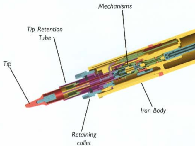
Cut-Away Drawing To show general principles or ProPiezo
